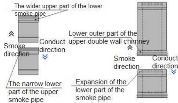
Drawing 3. Double wall chimney installation
